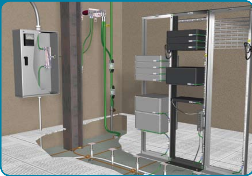
Figure 5. Bonded data center
