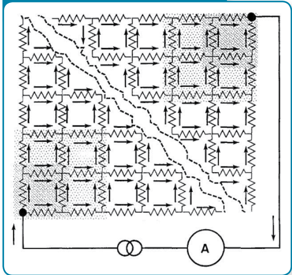
Figure 3. Top view of electrical schematic of an MCBN. Adapted from IEEE 1100, 2005, Figure 4-68. Current density is greatest as shading increases. Density becomes constant across plane after its equipotential line is crossed.
