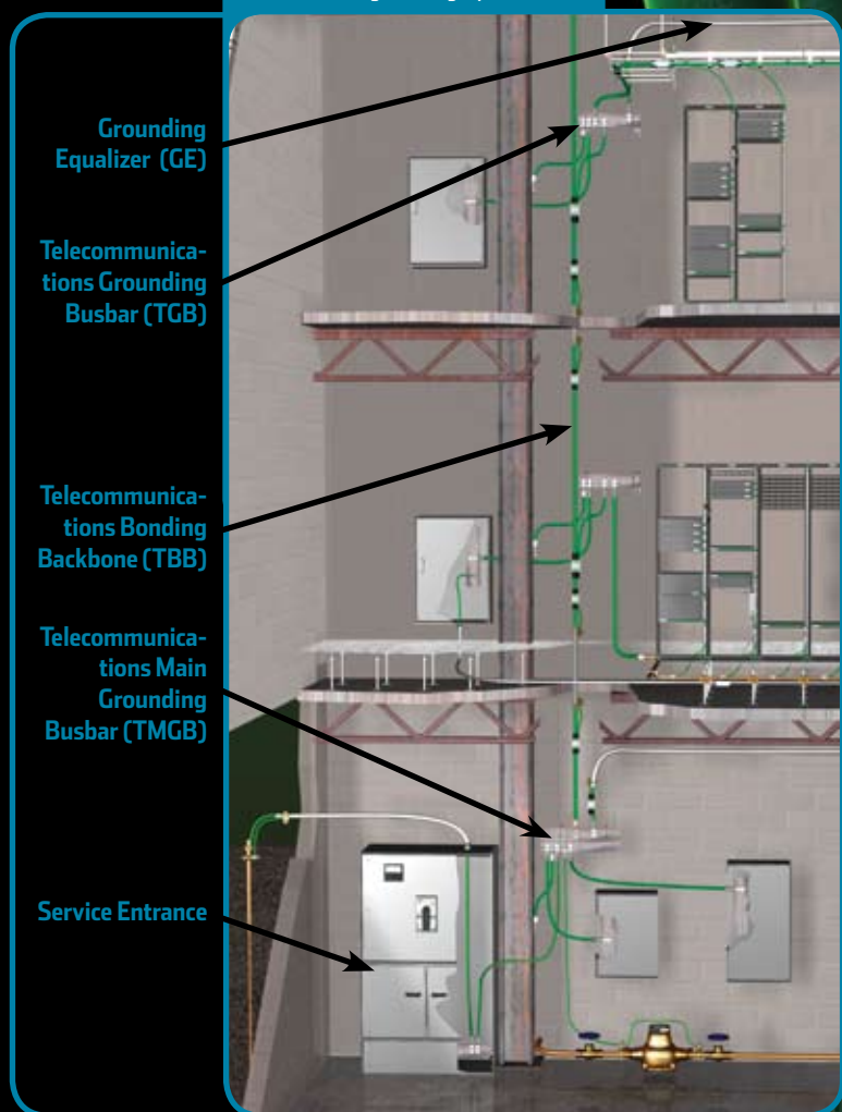
Figure 1. Telecommunications bonding backbone and grounding equalizer.
